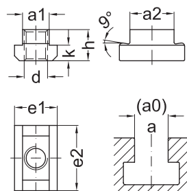
Riser T-Nuts 9° Hardness class 10 for Serie MQ 110/ 130/ 134
