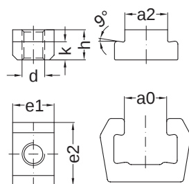
Riser T-Nuts 9° Hardness class 10 for Serie MQ 60/ 70/ 100/ 200/ 134 * for Serie MQ BG 8
